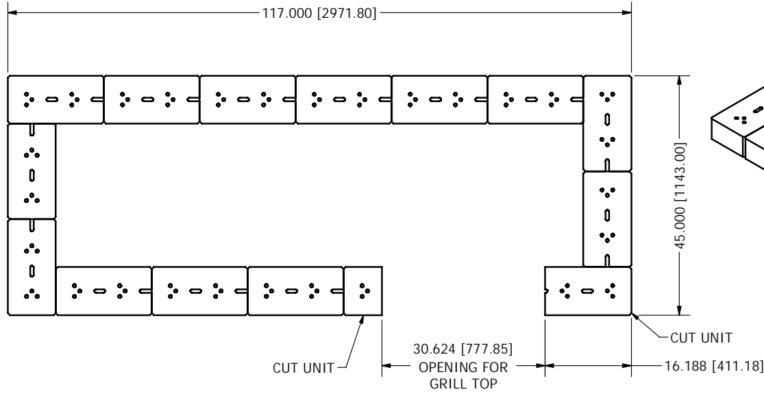
PLAN VIEW
