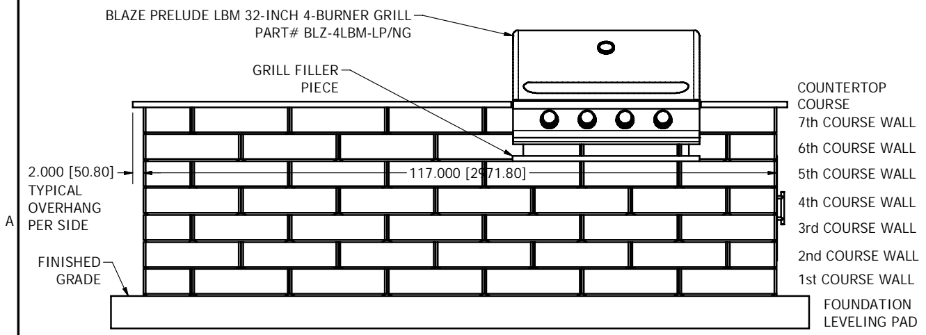
FRONT ELEVATION VIEW
