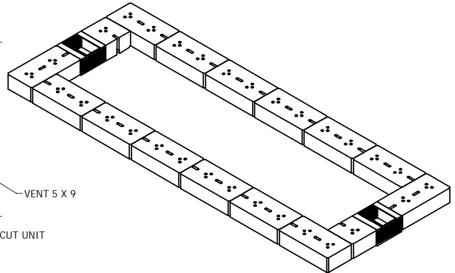
ISOMETRIC VIEW
